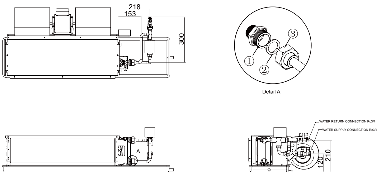
Figure 3 2-Way Valve
