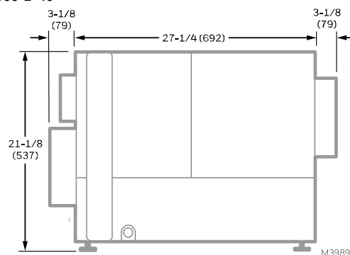
Fig. 1. Dimensions in in. (mm).
